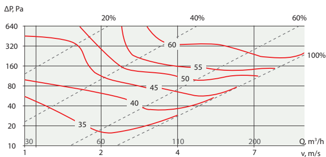
Diagram 1: Ø100 A – weighted sound power level L_{wa} , dB
