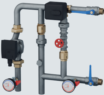
PPU – pipework package unit
